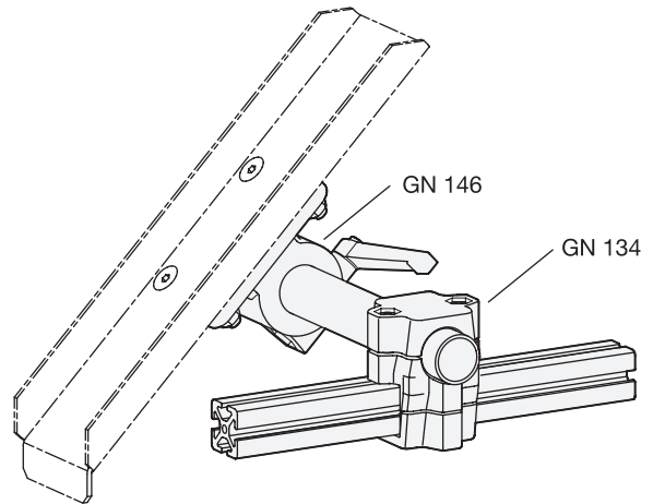
Workpiece chute Transfer to aluminum profile system
