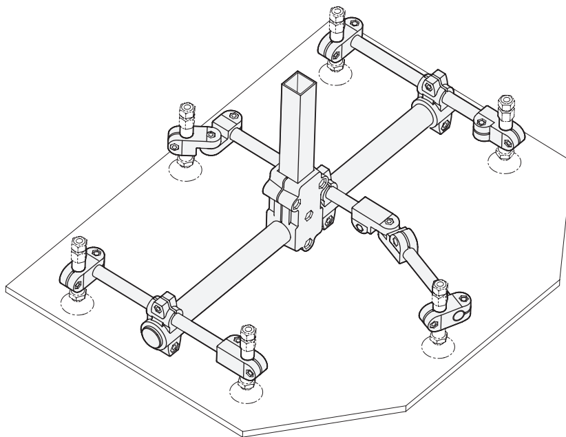
Vacuum gripper for plates
