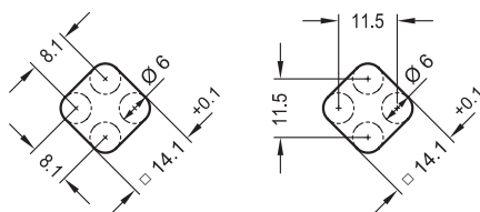
Installation hole for drilling or milling
