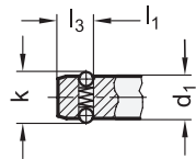
Pin Ø 10 / 12 Ball retainer both-sided
